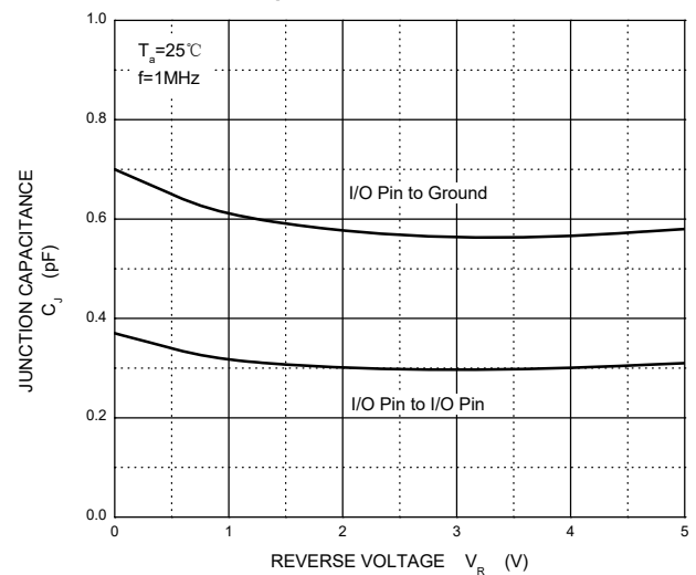
Capacitance Characteristics
